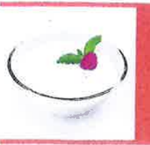
Quark nature
